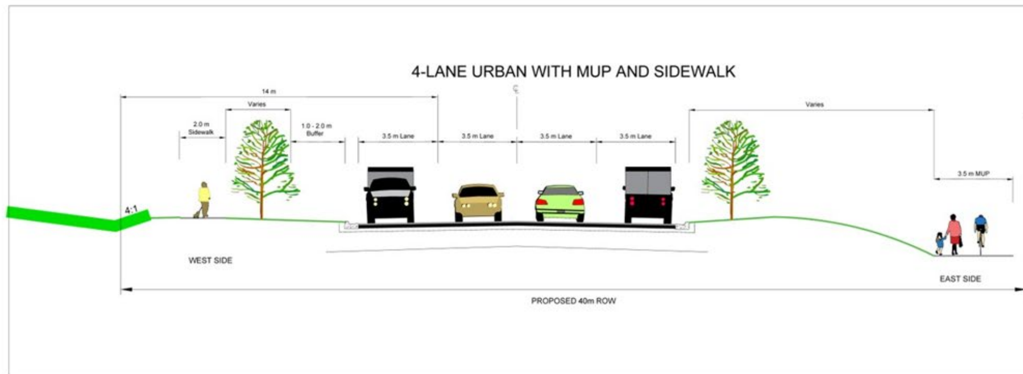
Figure 14: Preliminary 4-Lane Cross Section Alternatives - West Brant Access Road
