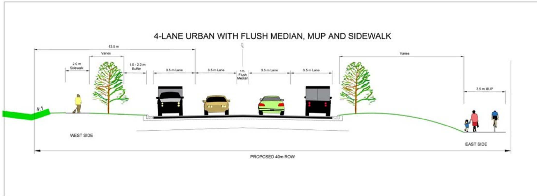
Figure 15: Preliminary 4-Lane with Flush Median Cross Section Alternatives - West Brant Access Road
