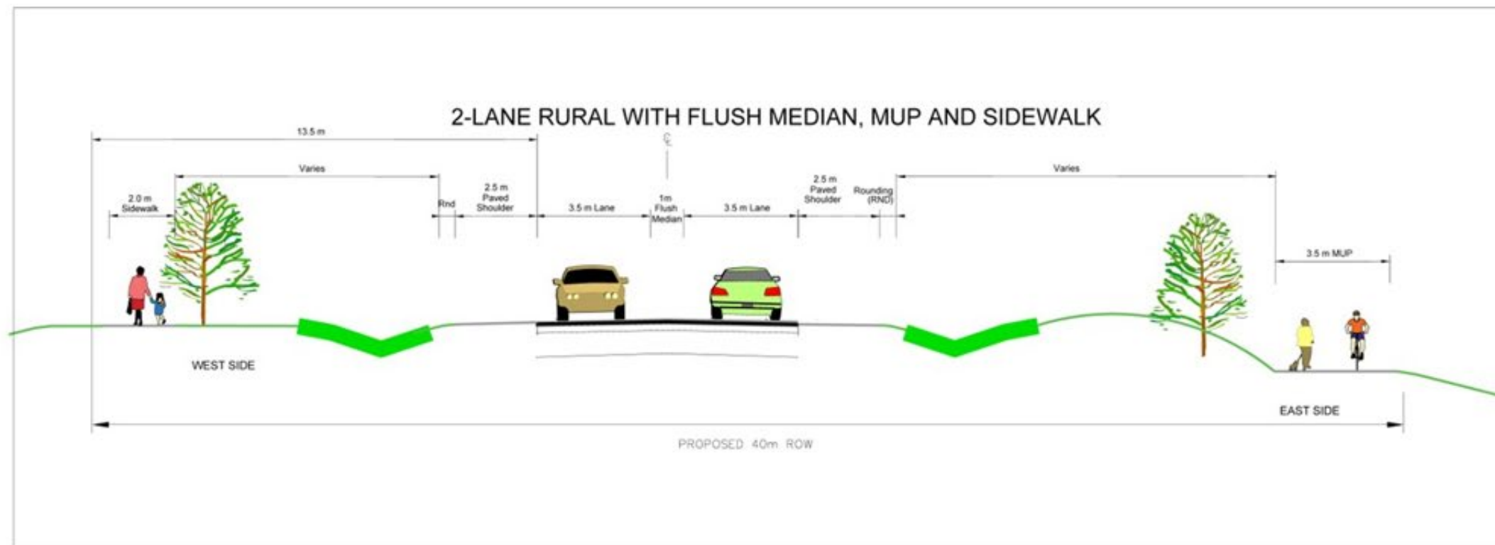
Figure 13: Preliminary 2-Lane Cross Section Alternatives - West Brant Access Road
