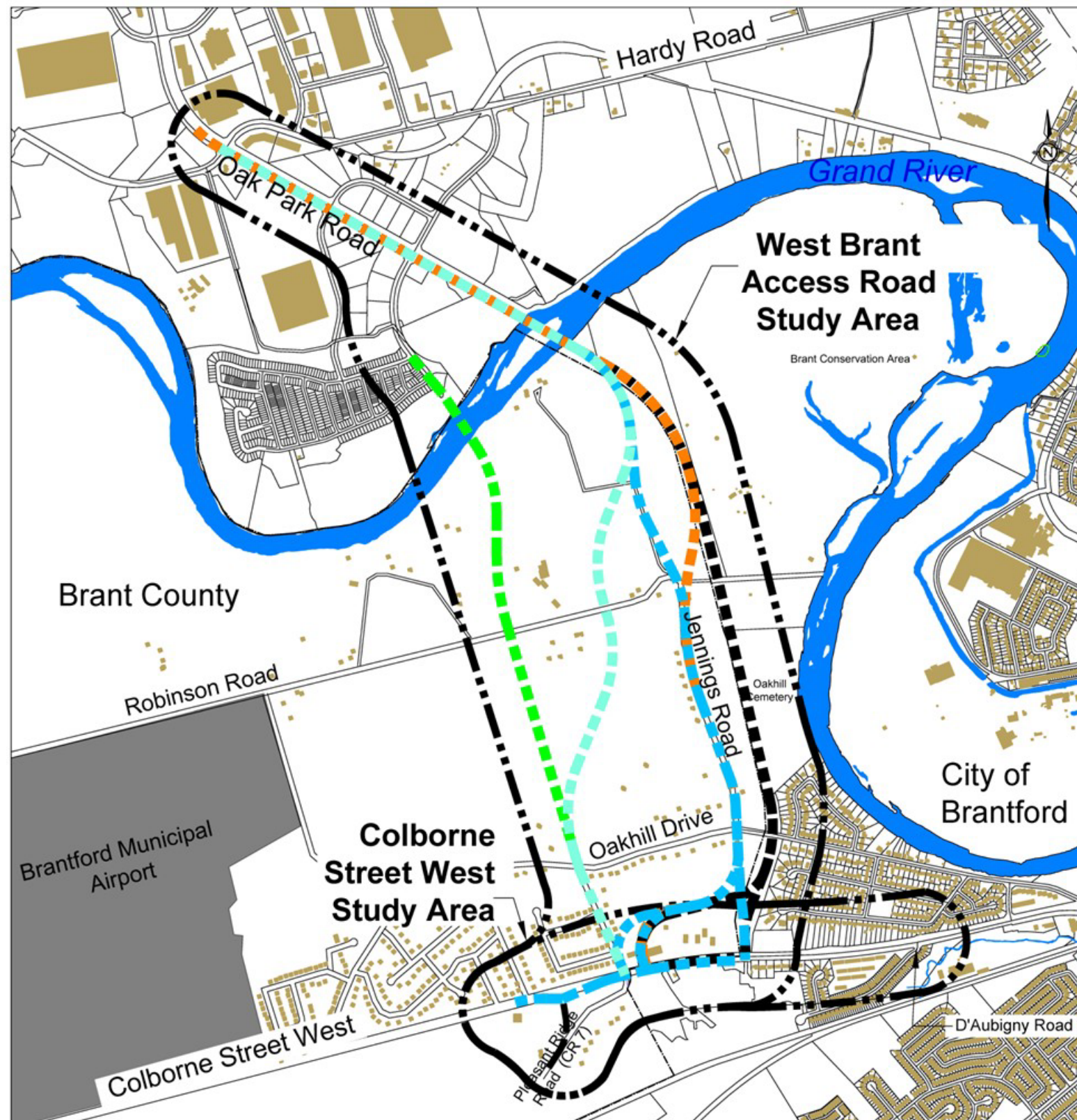
Figure 12: Preliminary Alignment Alternatives
