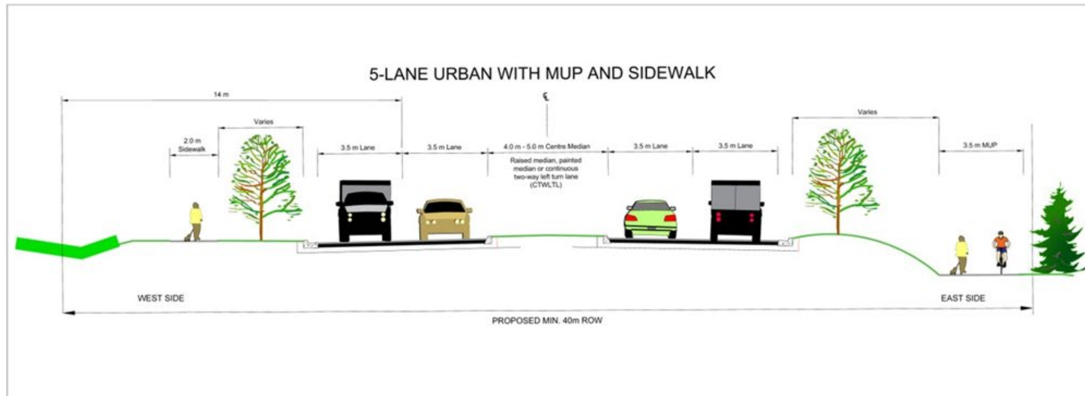
Figure 16: Preliminary 5-Lane Cross Section Alternatives - West Brant Access Road
